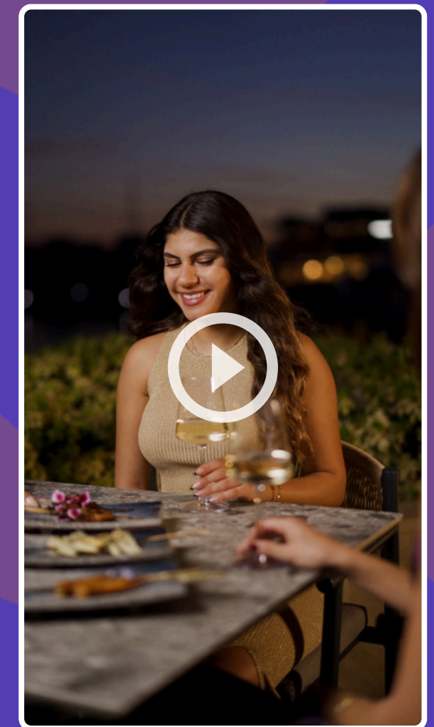
Malloc Campaign
