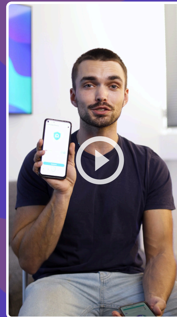
Malloc Campaign
